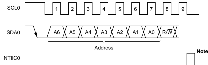
Figure 18-9. Address
