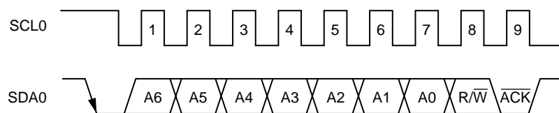
Figure 18-11. \overline{\text{ACK}} Signal
