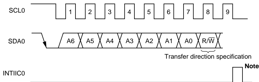
Figure 18-10. Transfer Direction Specification
