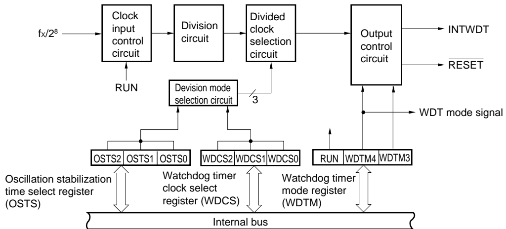
Figure 11-1. Watchdog Timer Block Diagram
